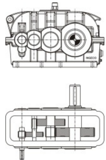
QUADRUPLE REDUCTION HELICAL GEAR BOX IDN / IDH In:- 112 to 630
