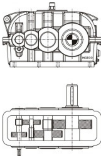
TRIPLE REDUCTION HELICAL GEAR BOX ICN / ICH In:- 14 to 112
